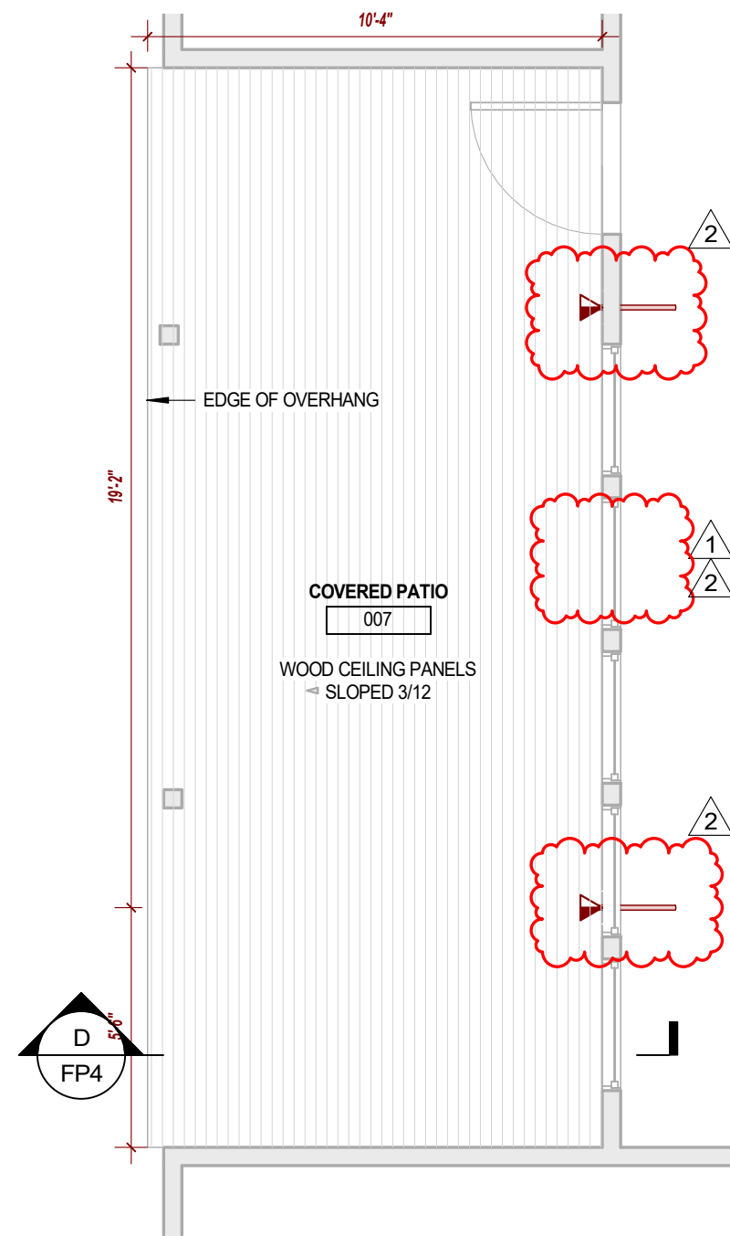
COVERED PATIO - RCP SCALE: 1/4" = 1'-0" NORTH
