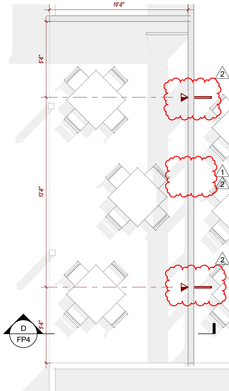
COVERED PATIO - FLOOR PLAN SCALE: 1/4" = 1'-0" NORTH
